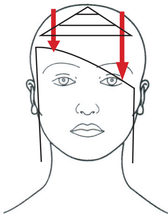
Asymmetric Fringe
